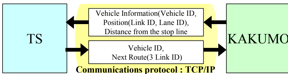
Figure 9. Communication data (in the KAKUMO area)
