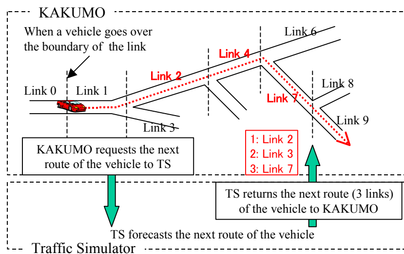
Figure 8. Mechanism of the route choice
