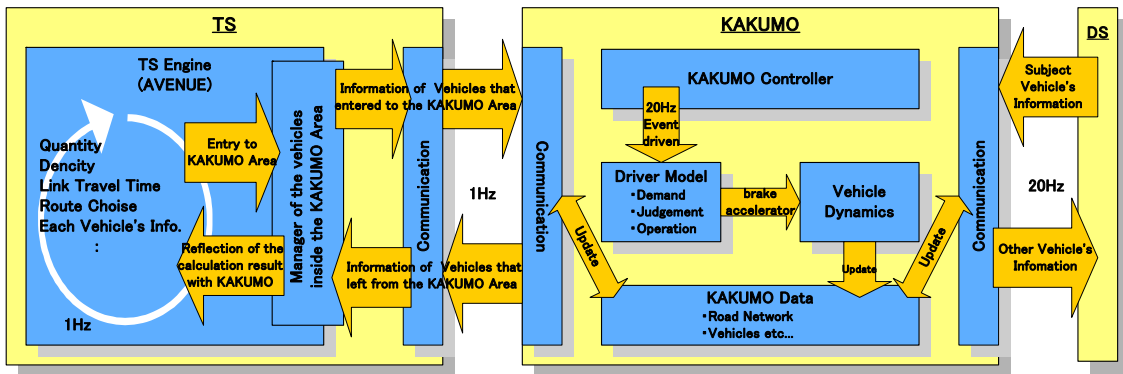
Figure 5. Data flow in VEL
