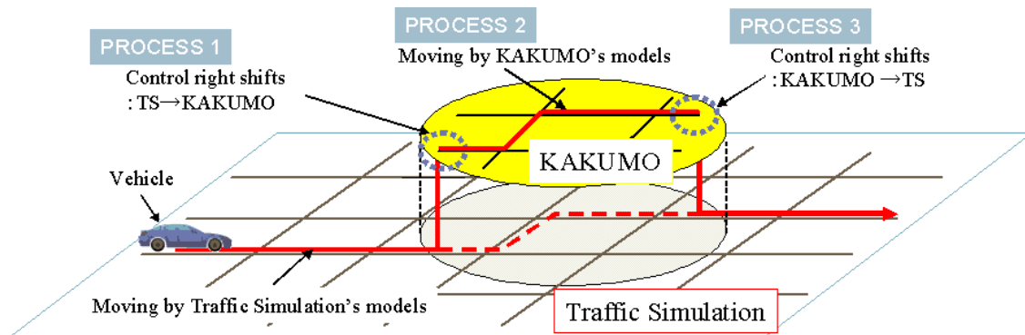
Figure 6. Three processes of Vehicle Motion
